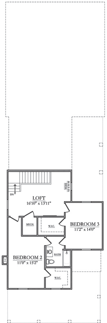
SECOND FLOOR
