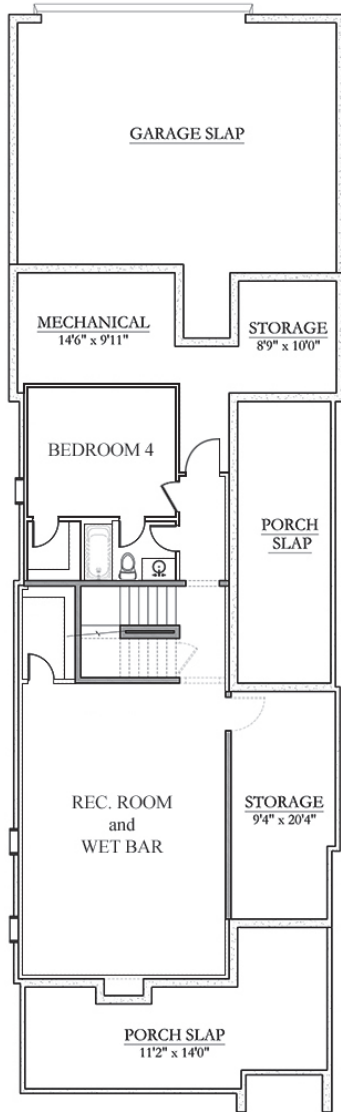
BASEMENT FLOOR
